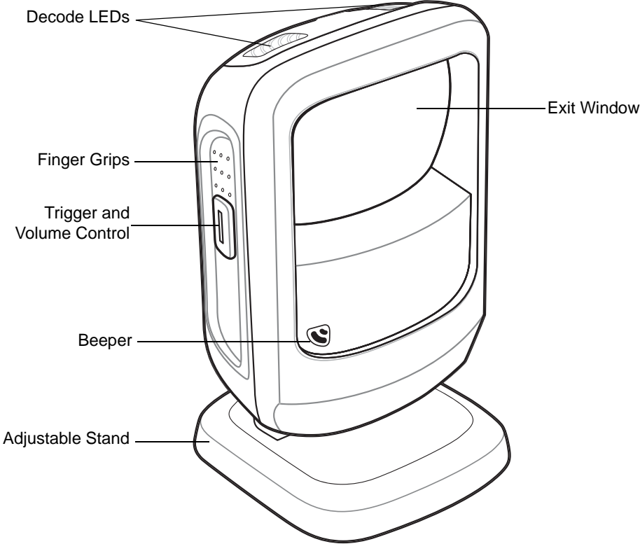
Figure 2-1 Parts
